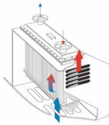
transverse installation
